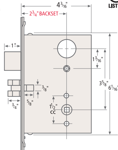
2 3 / 4 " Backset Lock
